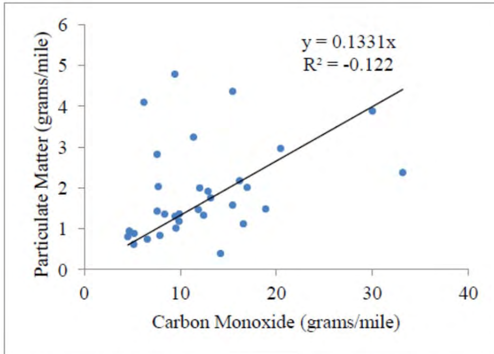
Figure 17 – Cycle-specific PM against CO for tests on vehicles with Pre 1994 engines evaluated at 56,000 lb inertial weight over the UDDS driving schedule.
