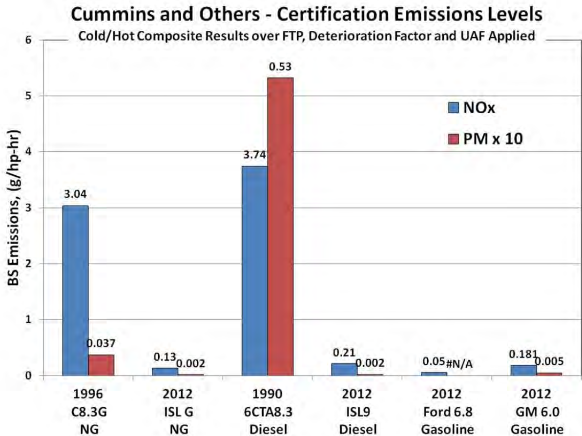
Figure 9: Cummins diesel and natural gas engines and other manufacturers' gasoline engines emissions over US Federal Certification Test cycle. (Wall (2012))
