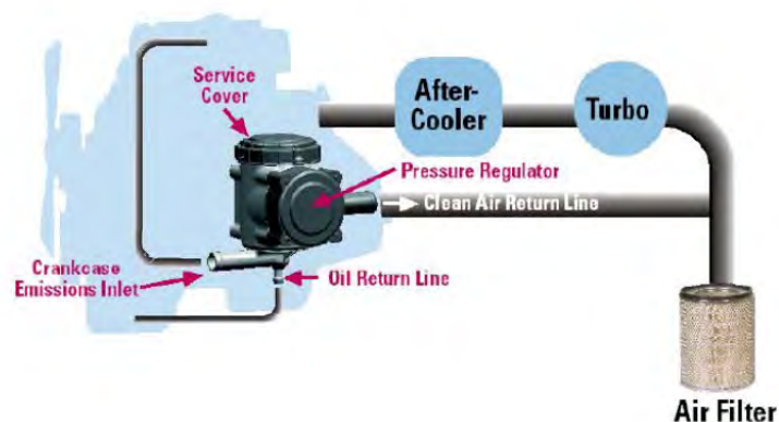
Figure A1-7: Closed crankcase emission control system
