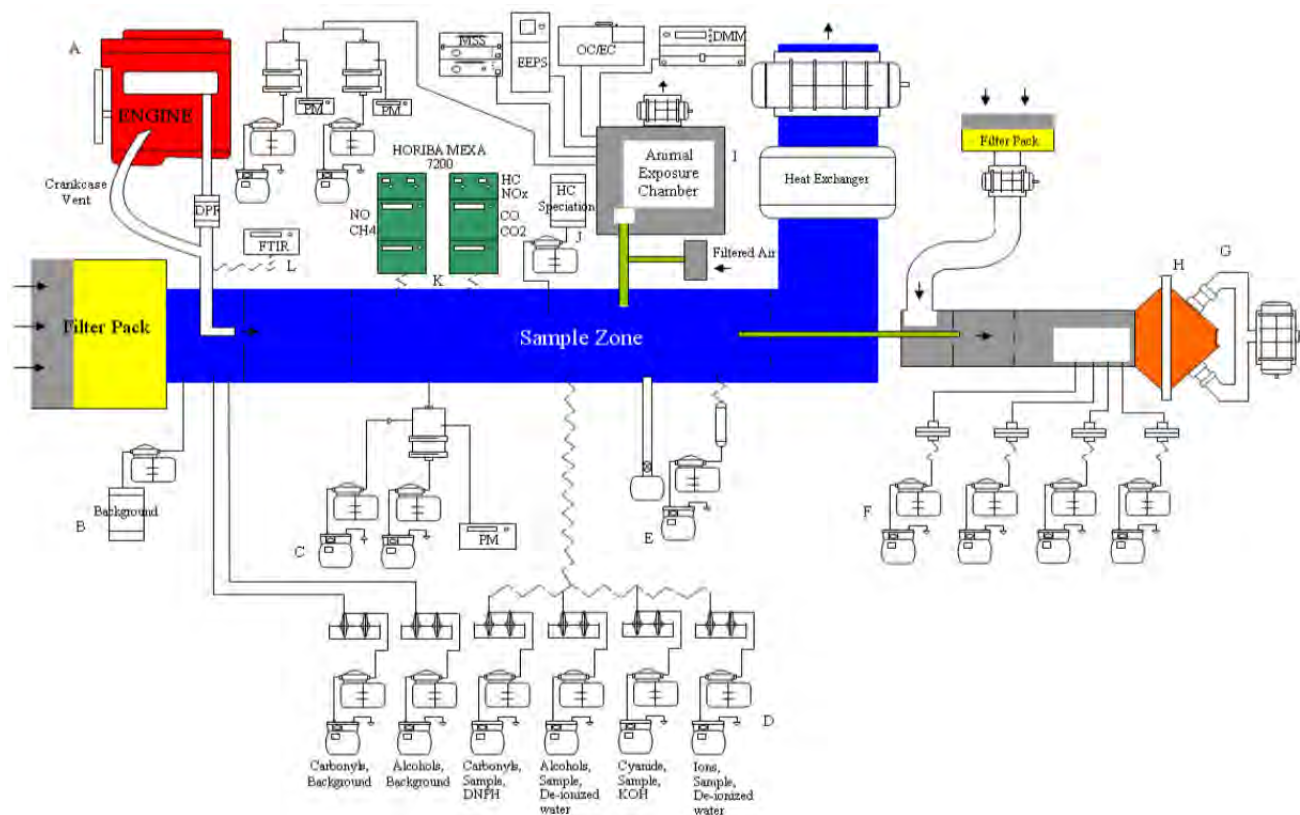
Figure A2-5: Overall experimental setup for the ACES program (Figure 1 from Khalek et al. (2011))
