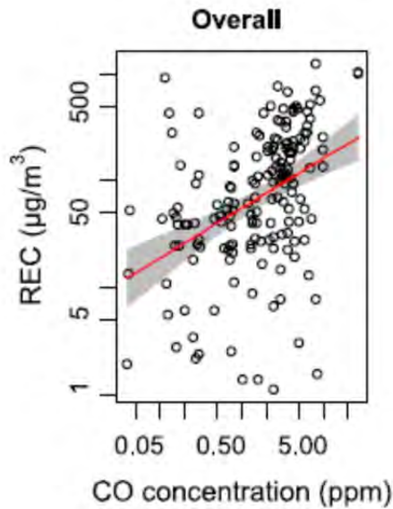
Figure 28: Scatter plot and regression analysis between natural-log transformed (Ln) CO and REC measurements for all mining facilities combined (from Fig.2, Vermeulen et al. (2010a), (2010b))
