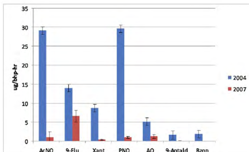
Figure 15: Concentration of oxy-PAH from a 2004 model engine without exhaust after-treatment compared to 2007 model with contemporary controls (Liu et al. (2010)).
