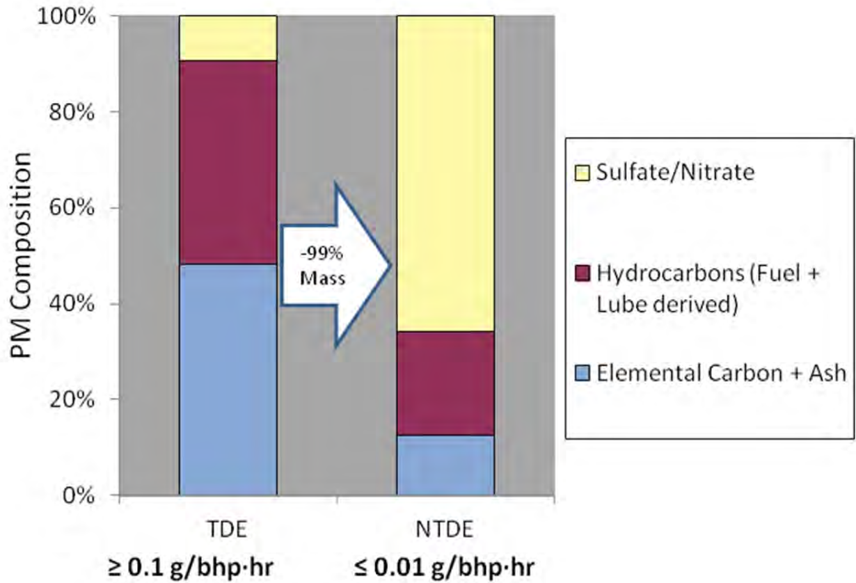
Figure 11: More than 99% PM reduction with DPF and a substantial shift in chemical composition. EC is substantially reduced in NTDE and sulfate dominates. (data from Liu (2009a))
