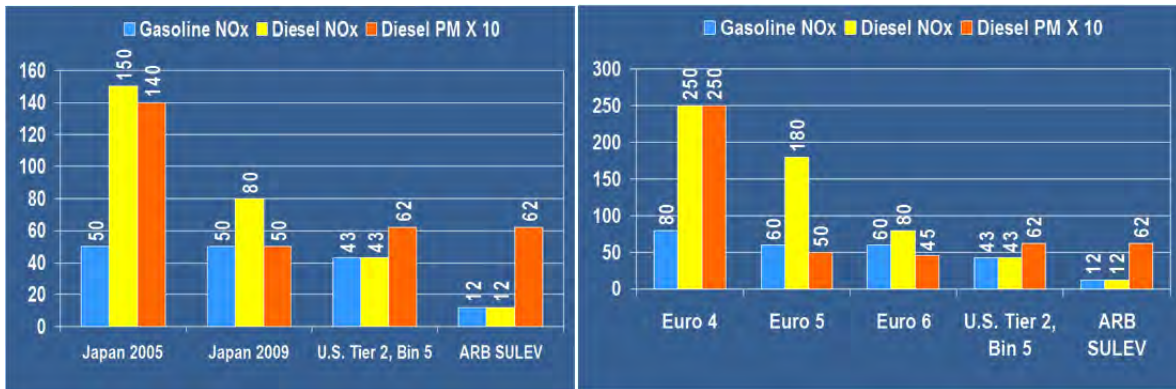
Figure A1-2: Emissions regulations for light-duty engines
