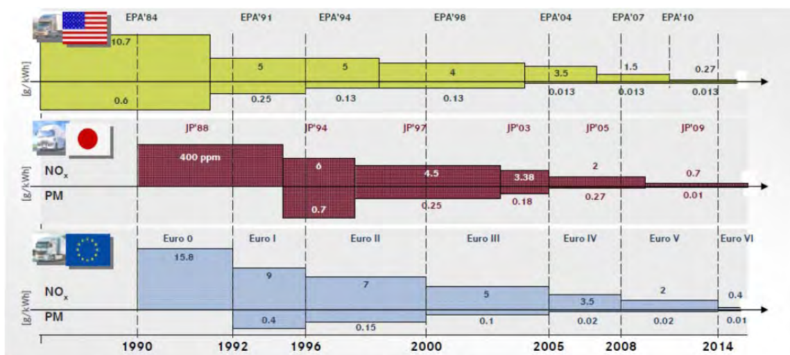
Figure A1-1: Emissions regulations for heavy-duty diesel engines [1]
