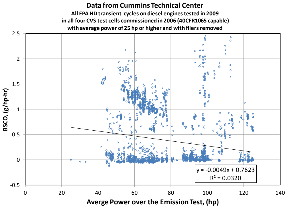
Figure 26: CO-average horsepower linear correlation for all Cummins engines with average hp above 25 tested over the EPA HD transient cycles in four CVS cells at the Cummins Technical Center in 2009 (Martin (2012))
