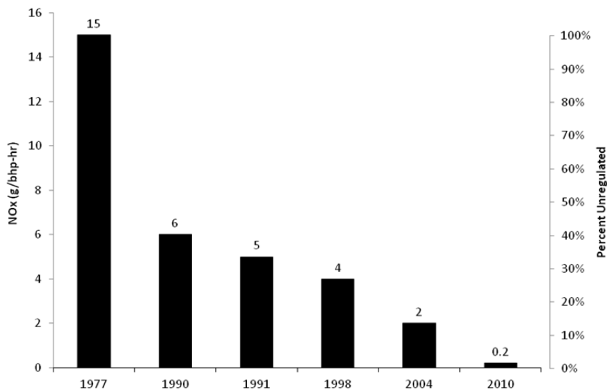
Figure 3: U.S. EPA NOx emission standards for heavy-duty on-road diesel engines in grams per brake horsepower-hour (g/bhp-hour) (left axis) and as a percentage of “unregulated” emissions (right axis).
