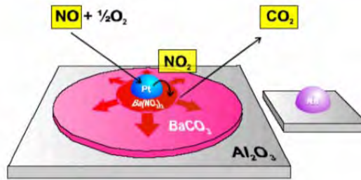
Figure A1-11: NO x trapping mechanisms under lean operating conditions.
