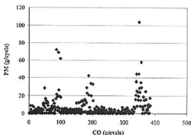
Figure 22: Poor correlation between PM and CO (Xu et al. (2005))
