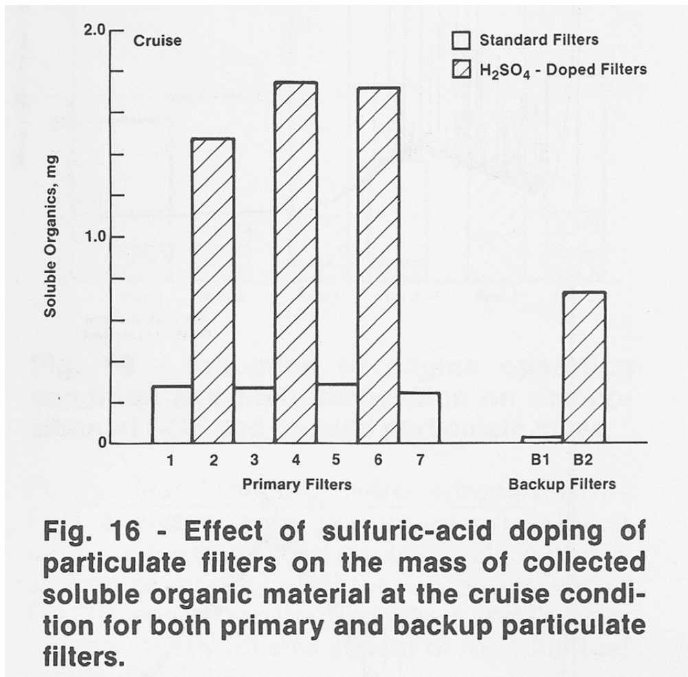
Figure A2-3: Effect of sulfuric-acid doping of particulate filters on the mass of collected soluble organic material at the cruise condition for both primary and backup particulate filters (Figure 16, Wall (1984))
