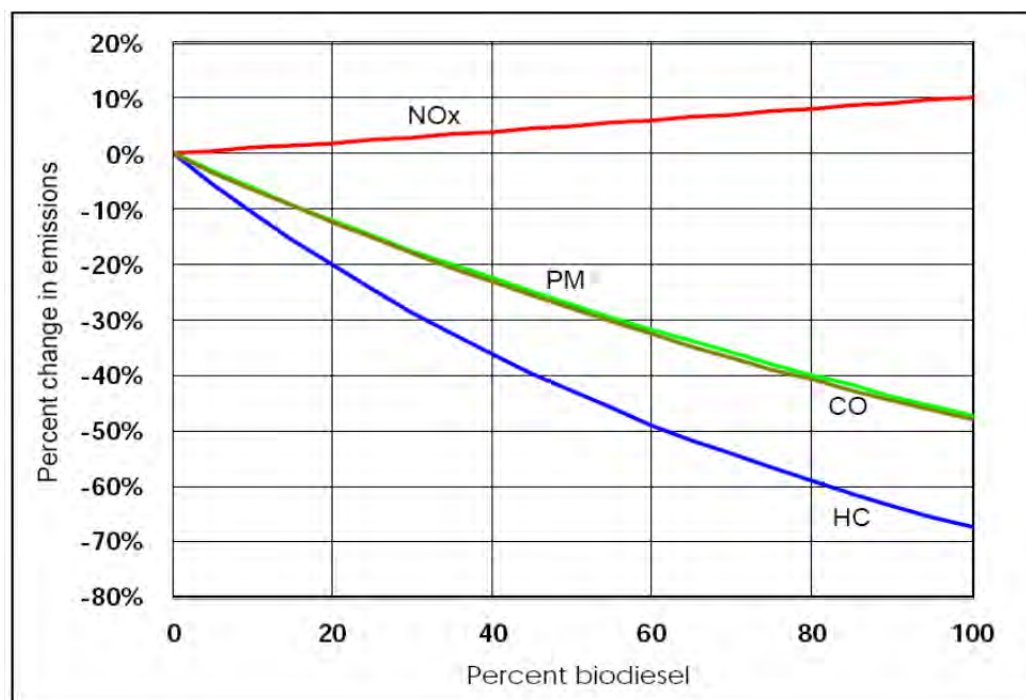
Figure A1-14: Average emission impacts of biodiesel for heavy-duty highway engines [1]
