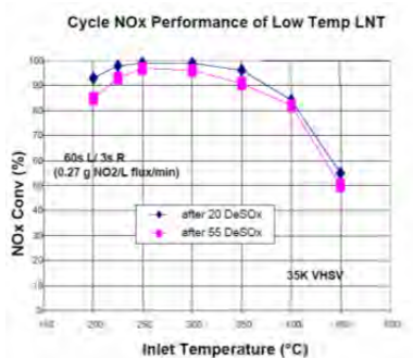
Figure A1-13: Durability of advanced LNTs can be maintained over many high temperature desulfation cycles.
