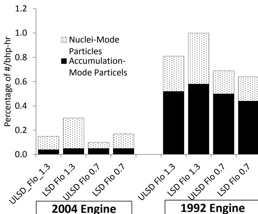
Figure 19: Normalized total PN emissions during the entire U.S. FTP cycles for a 1992 TDE and a 2004 engine equipped with an EGR system operating on either ULSD (<15ppm S) and low-sulfur (308ppm S) diesel fuel, with flow rates of 0.7 or 1.3m 3 /S (Liu et al. (2007)).
