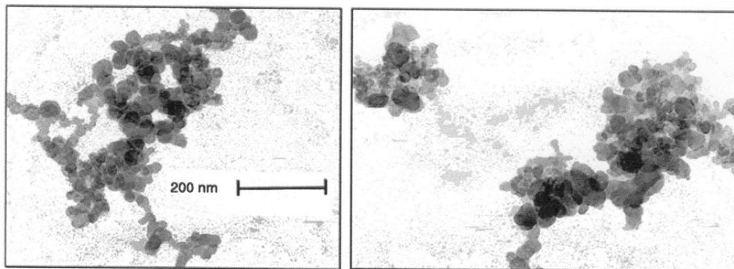
Figure 1: Two scanning electron micrograph (SEM) images of traditional diesel exhaust (TDE) PM (reproduced from Tschoeke et al. (2010)).
