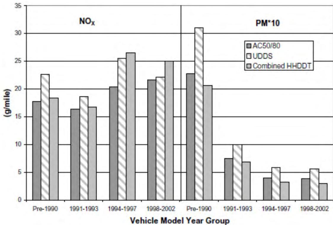
Figure 26: Comparison of the AC50/80, UDDS, and the combined HHDDT for NO x and PM emissions.
