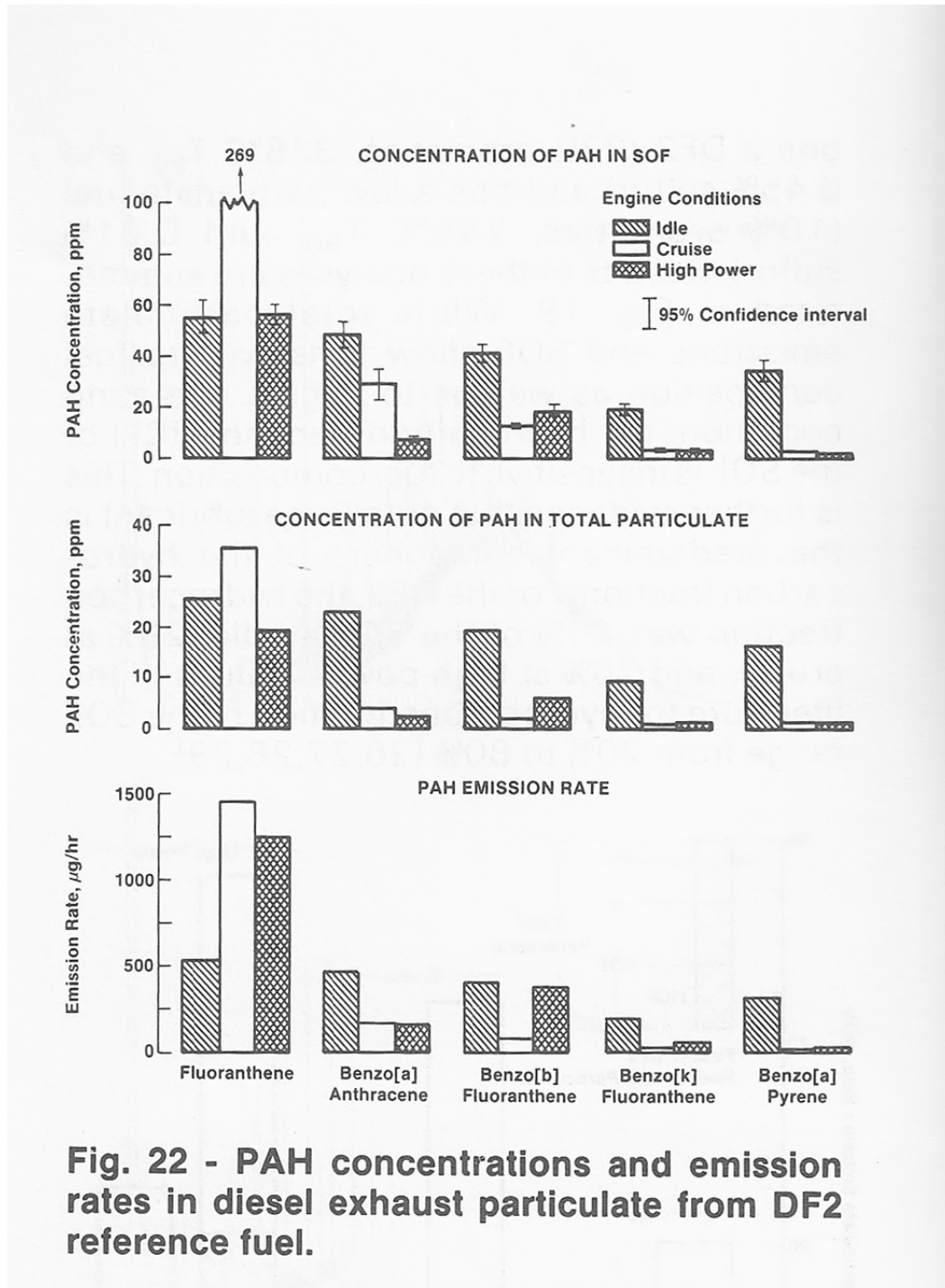
Figure 5: Impact of engine operating condition on TDE PAH emissions (appears as Figure 22 in Wall and Hoekman (1984))
