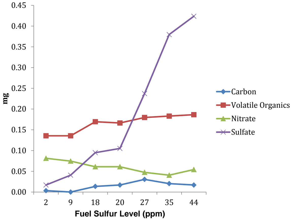
Figure 12: Measured PM emissions (carbon, volatile organics, sulfate and nitrate) continuously regenerating DPF from a heavy duty diesel engine as a function of fuel sulfur content (adapted from Figure 3 in Kittelson et al. (2006a)).
