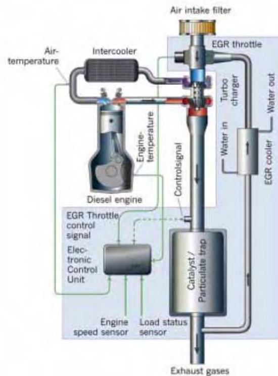
Figure A1-8: Low Pressure EGR plus DPF
