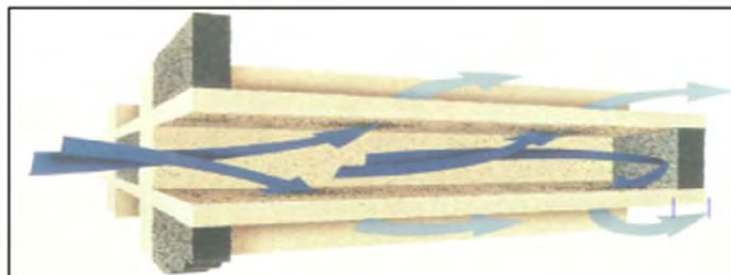
Figure A1-4: Exhaust gas flow through a wall-flow filter channel
