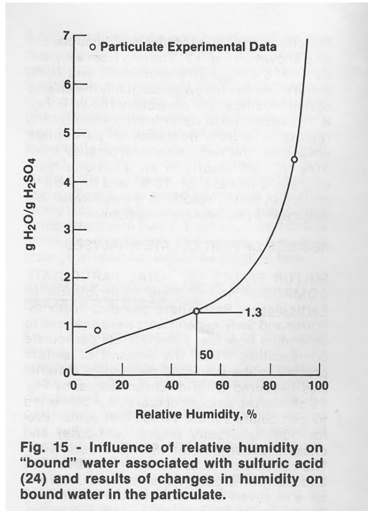
Figure A2-4: Influence of relative humidity on mass of “bound” water associated with sulfuric acid and contributing to total PM. (Figure 15, Wall (1984))
