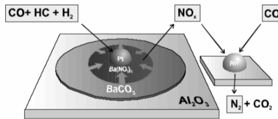
Figure A1-12: NO x trap regeneration occurs under brief periods of rich operation.
