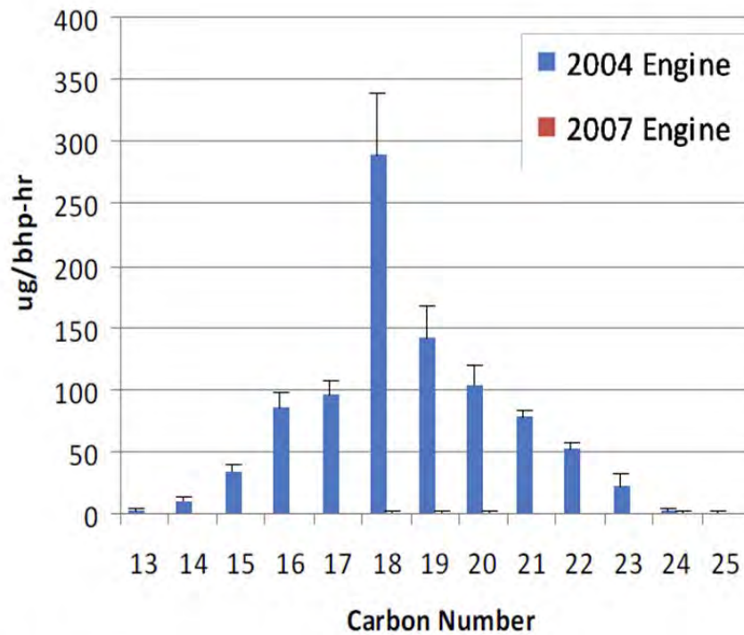
Figure 13: Reduced concentrations of PAH emissions from a 2007 diesel engine with contemporary emission controls compared to emissions from a 2004 engine without contemporary emission controls (Liu et al. (2010)).
