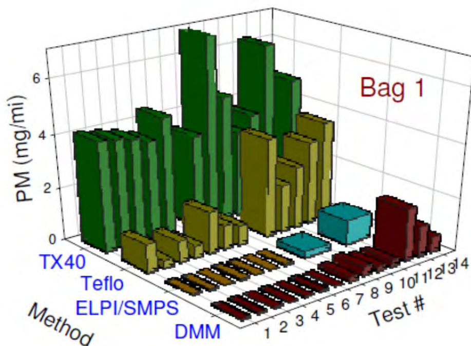
Figure A2-2: PM Mass Artifact due to Adsorption of Semi-Volatiles (Chase and Duszkievicz (2004))
