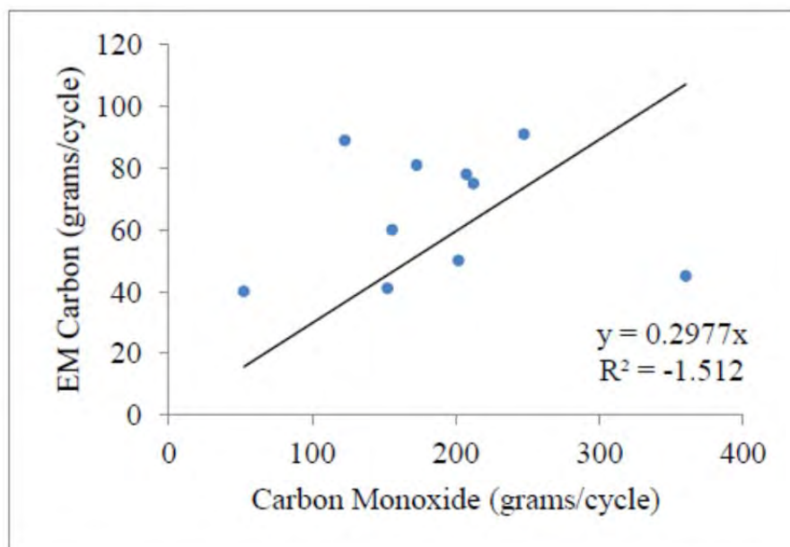
Figure 35 – Cycle-specific EC fraction of PM against CO for trucks with 1950-1975 model year diesel engines.
