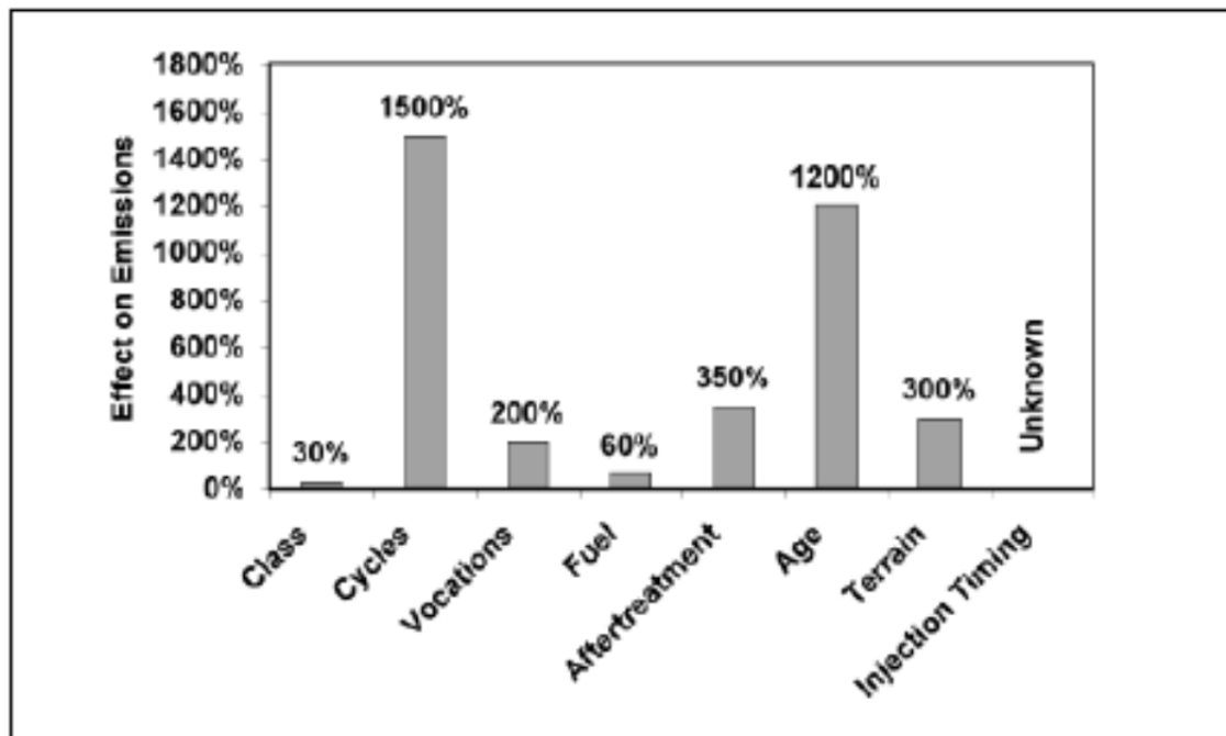
Figure 7: Relative impact of operating variables on PM emissions (appears as Figure 6 in Clark et al. (2002))
