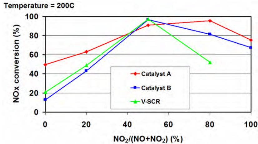
Figure A1-9. Catalyst A: Cu-zeolite and Catalyst B: Fe-zeolite are compared to a vanadia-based SCR catalyst with respect to NO 2 sensitivity
