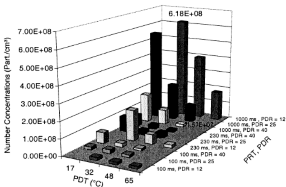
Figure A2-1: Impact of Residence Time (PRT), Dilution Ratio (PDR) and Dilution Temperature (PDT) on Diesel Particle Number Emissions (Watts and Kittelson (2002))
