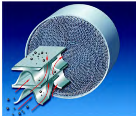
Figure A1-6: Metallic partial flow filter made up of corrugated metal foil and layers of porous metal fleece
