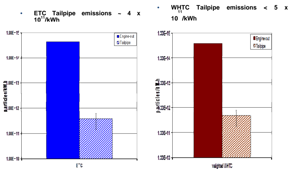
Figure A1-5: Particle number measurements with and without wall-flow DPF controls on heavy-duty engines using the PMP guidelines [11]
