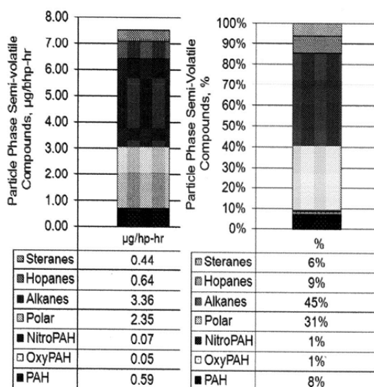
Figure 16: Average particle phase semi-volatile emission rate and composition for all twelve repeats of the 16-hour cycles using all four ACES engines (Khalek et al. (2011)).
