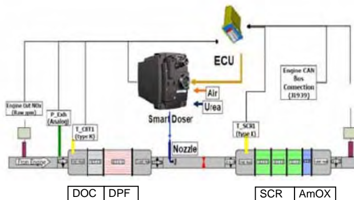
Figure A1-10: Diagram showing SCR (green) catalyst downstream of DOC (light gray)/DPF (pink) catalyst, urea dosing nozzle. The blue section represents an ammonia clean-up catalyst. Some of the types of monitors and controls feeding back to the control unit are also shown.
