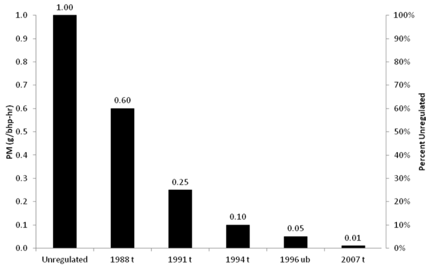
Figure 2: U.S. EPA PM emissions standards for heavy-duty on-road diesel trucks (t) or urban buses (ub) in grams per brake-horsepower-hour (g/bhp-hr) (left axis) and as % of “unregulated” engine emissions (right axis) 2
