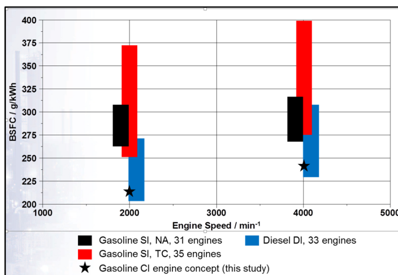
Figure 25 Break specific fuel consumption of YE2012 state of the art engines including the GCI concept
