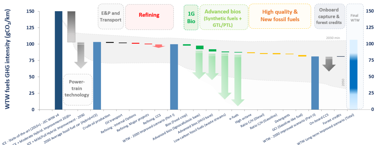
Figure 6 Concawe Low Carbon Pathways model – High level assessment (Passenger cars. C-segment).
