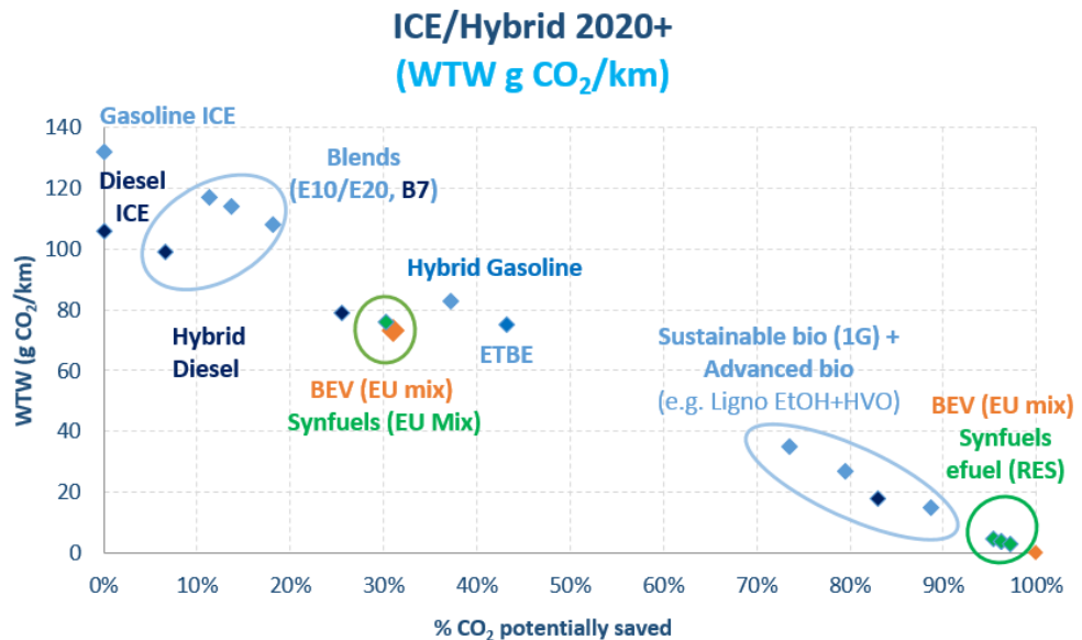
Figure 18 Comparison of WTW impact of different powertrains combined with liquid fuels and BEVs
