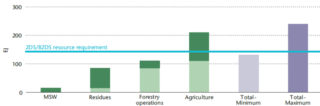
Figure 21 Potential sustainable biomass resources (Worldwide)
