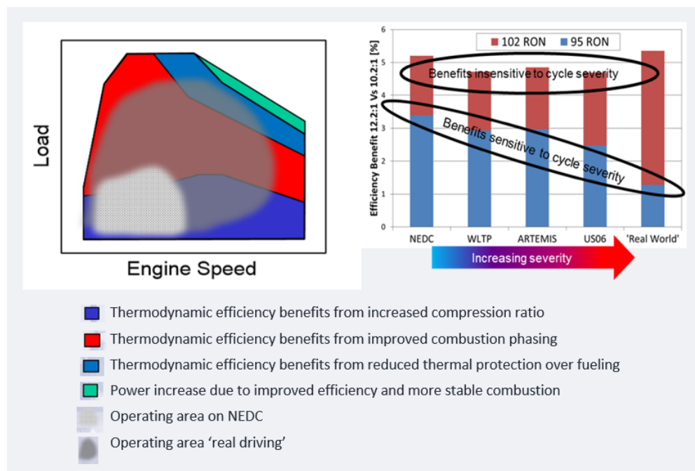
Figure 24 Mechanisms and efficiency improvements
