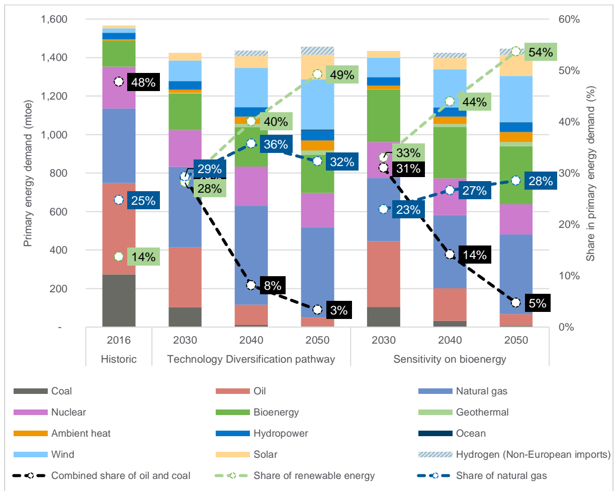
Figure 58. Evolution of total primary energy demand in the Technology Diversification pathway and the sensitivity on bioenergy potential, 2016 to 2050
