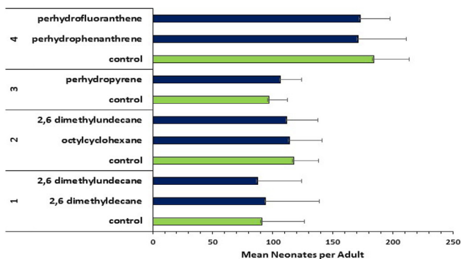
Fig. 2. Daphnia magna mean neonate production per adult in control (green bars) and hydrocarbon dosed treatments (blue bars); Observed reproduction in hydrocarbon test exposures was not statistically different ( p < 0.05 ) from corresponding controls. The numbers to the left of the figure denote the test number as described in Table S3. (For interpretation of the references to colour in this figure legend, the reader is referred to the Web version of this article.)
