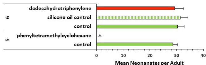
Fig. 3. Ceriodaphnia dubia mean neonate production per adult in control (green bars) and hydrocarbon dosed treatments (red bar); Asterisk denotes no data since complete adult mortality was observed precluding reproduction. The numbers to the left of the figure denote the test number as described in Table S3. (For interpretation of the references to colour in this figure legend, the reader is referred to the Web version of this article.)
