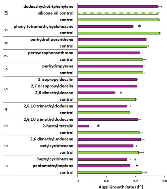
Fig. 1. Algal growth rates in control (green bars) and hydrocarbon dosed treatments (purple bars); Asterisks indicate growth rates are statistically different ( p < 0.05 ) from corresponding controls. The numbers to the left of the figure denote the test number as described in Table S3. (For interpretation of the references to colour in this figure legend, the reader is referred to the Web version of this article.)
